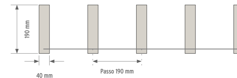
Parete divisoria aperta Open partition wall
