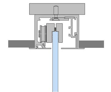
Binario FILOMURO WALL FILOMURO WALL track
